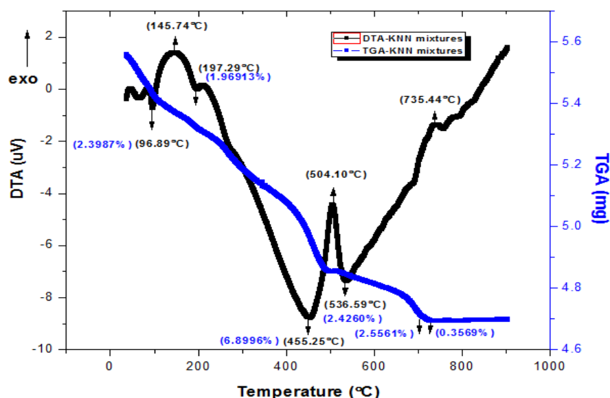
Fig. 2. TGA and DTA curves of the KNN mixtures.
