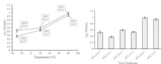
Figure 22 Fracture energy as a function of temperature and strain rate [99].
