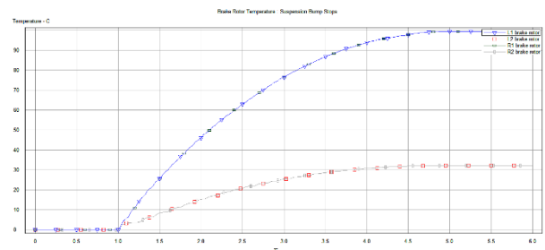
Figure 25: Brake Rotor Temperature C-Time(s) "Carsim_ABS_ON"
