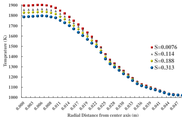
Figure 13: Soot effect on Radial Temperature variation
