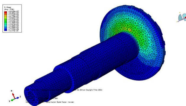
Fig9. Stress analysis of stable secondary half pulley with ABAQUS
