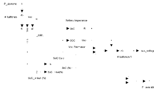
Fig6. The battery model in MATLAB/Simulink
