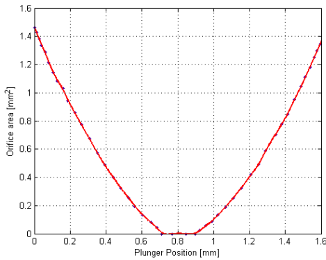
Fig2. Graph of clutch servovalve orifice area vs. plunger position.
